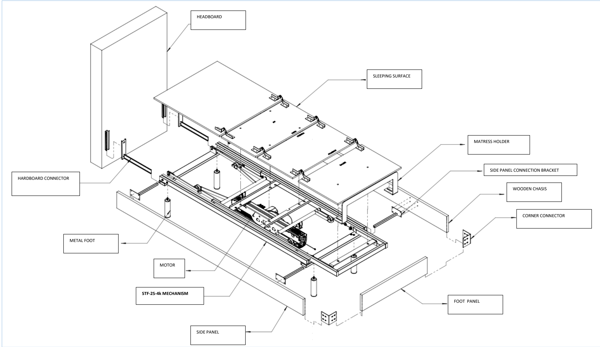
ASSEMBLY GUIDE EXAMPLE FOR STF-27-4K
