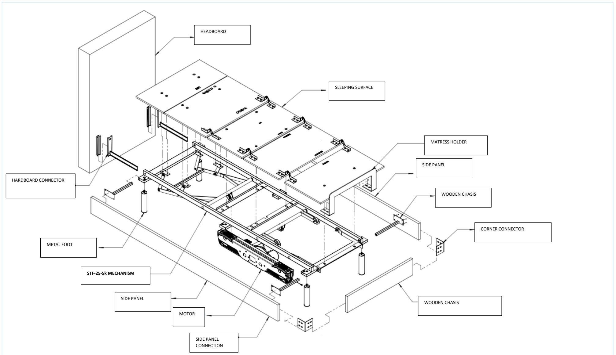
ASSEMBLY GUIDE EXAMPLE FOR STF-25-5K
