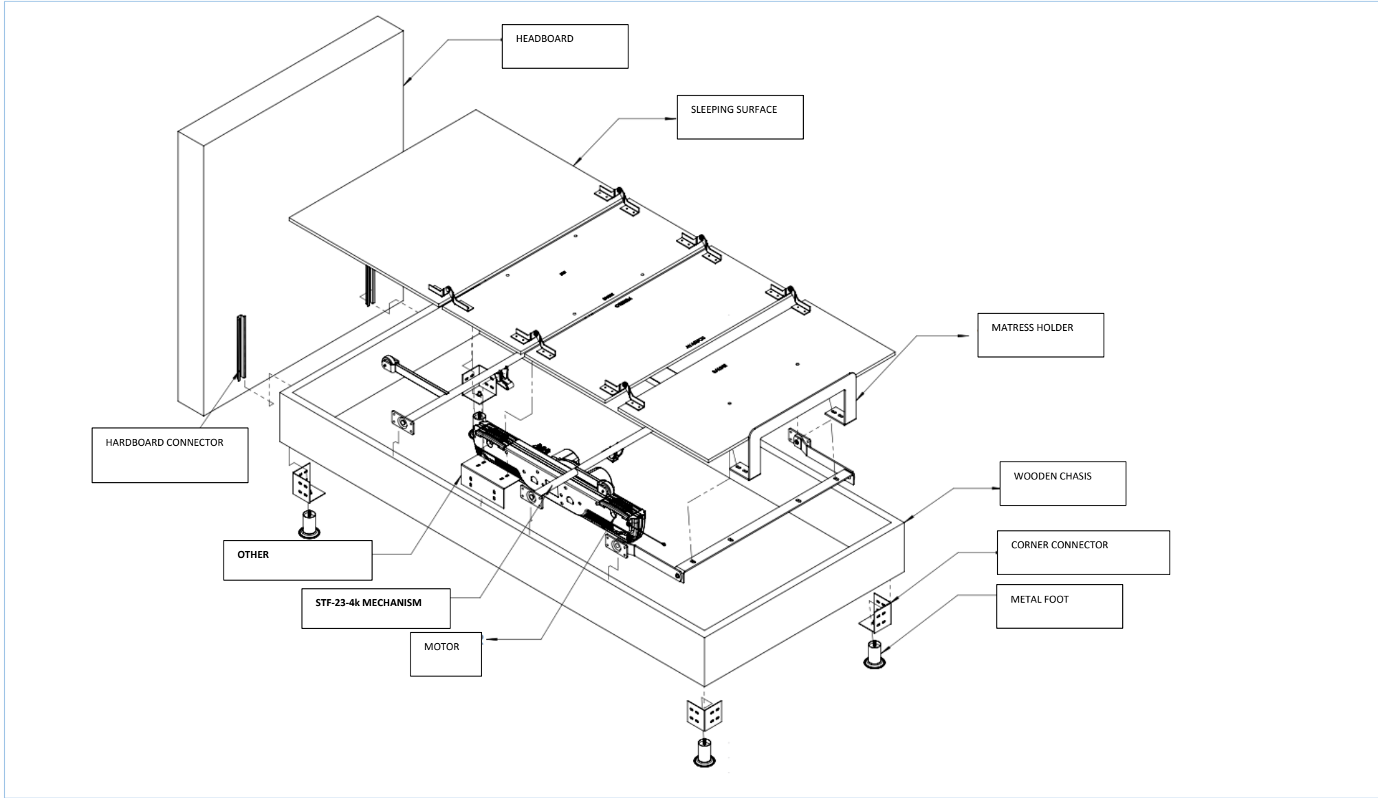
ASSEMBLY GUIDE EXAMPLE FOR STF-23-4K
